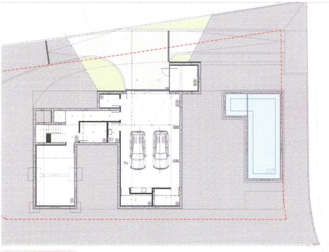
Cave | 151,80m 2
